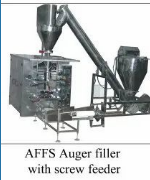
Automatic Foam Fill Seal Machine With Screw Feeder
